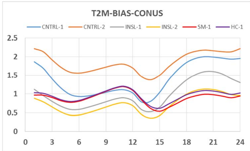
Figure 1 Average hourly bias values (K) for temperature at 2-m for various WRF simulations for the entire 12-km grid for 1-31 August 2012. Values calculated at all surface observing stations.
